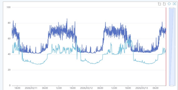
Example of data plot (LAeq, LA10 and LA90)
